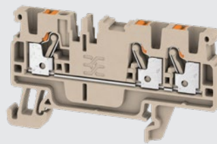
A typical Klippon® terminal block from Weidmüller, as it looks at the end of the process after coming out of the injection molding machine, including integrated metal parts.
