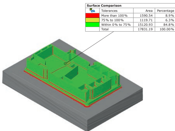
Fig. 5: The ATOS ScanBox digitizes all sides and surfaces, combines them and compares the captured data to the CAD model. Deviations are identified by false colors in dependence on the present spark gap
