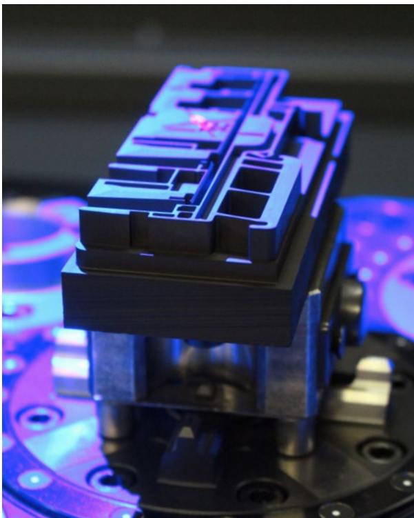
Fig. 1: The ATOS ScanBox measures even narrow and deep grooves in electrodes without trouble
