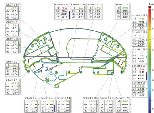
Fig. 14: Customized inspection report
