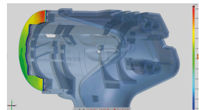
Fig. 4: The plane on the head of the drill cover is warped as shown in the color plot highlighting the deviations from CAD data.
