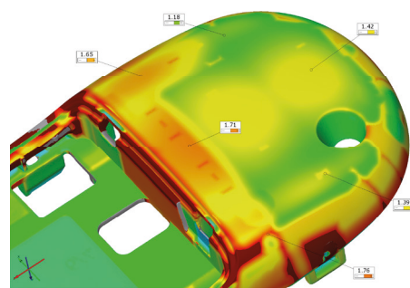
Fig. 7: Material thickness analysis in the ATOS Inspection Software
